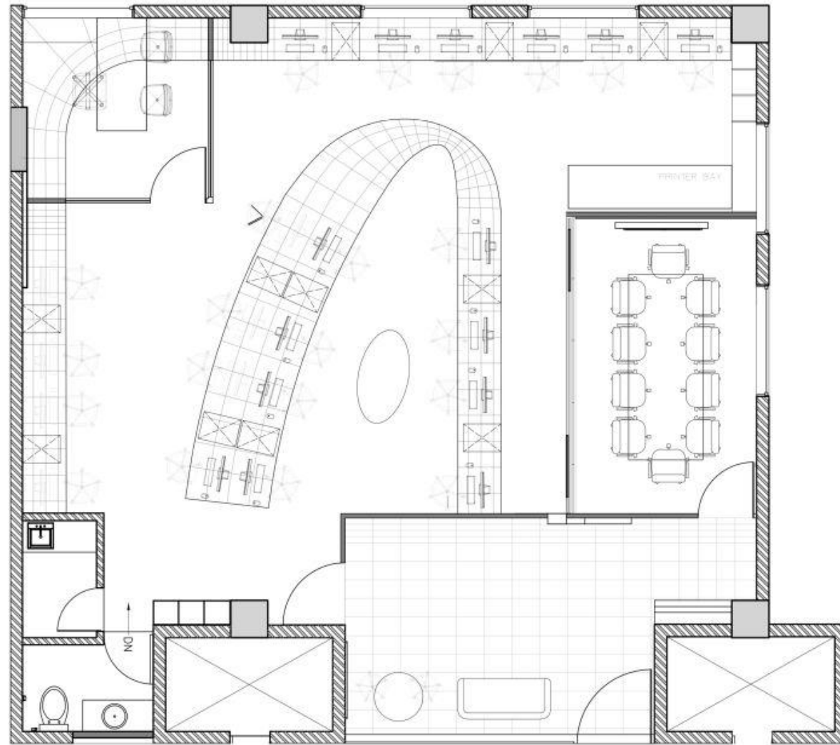
FLOOR LAYOUT
